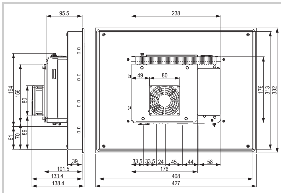
Fig. 58 Mechanical dimensions of the 15" devices in mm
