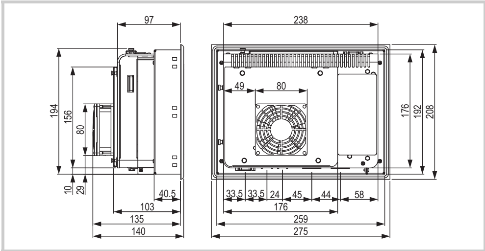
Fig. 55 Mechanical dimensions of the 8.4" devices in mm
