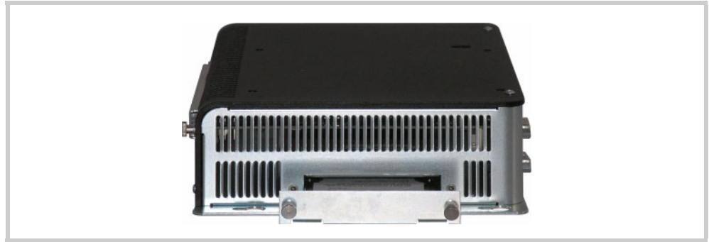
Fig. 29 Inserting a hard disk into the hard disk slot
