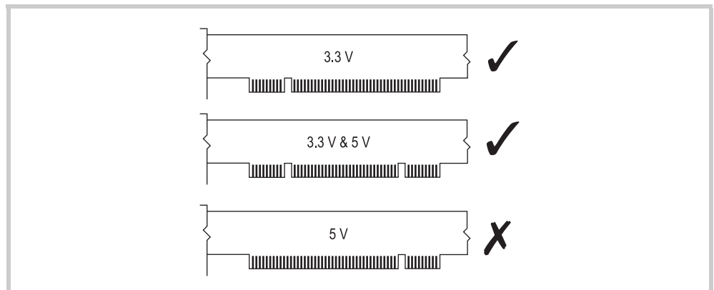
Fig. 17 Usable PCI expansion cards
