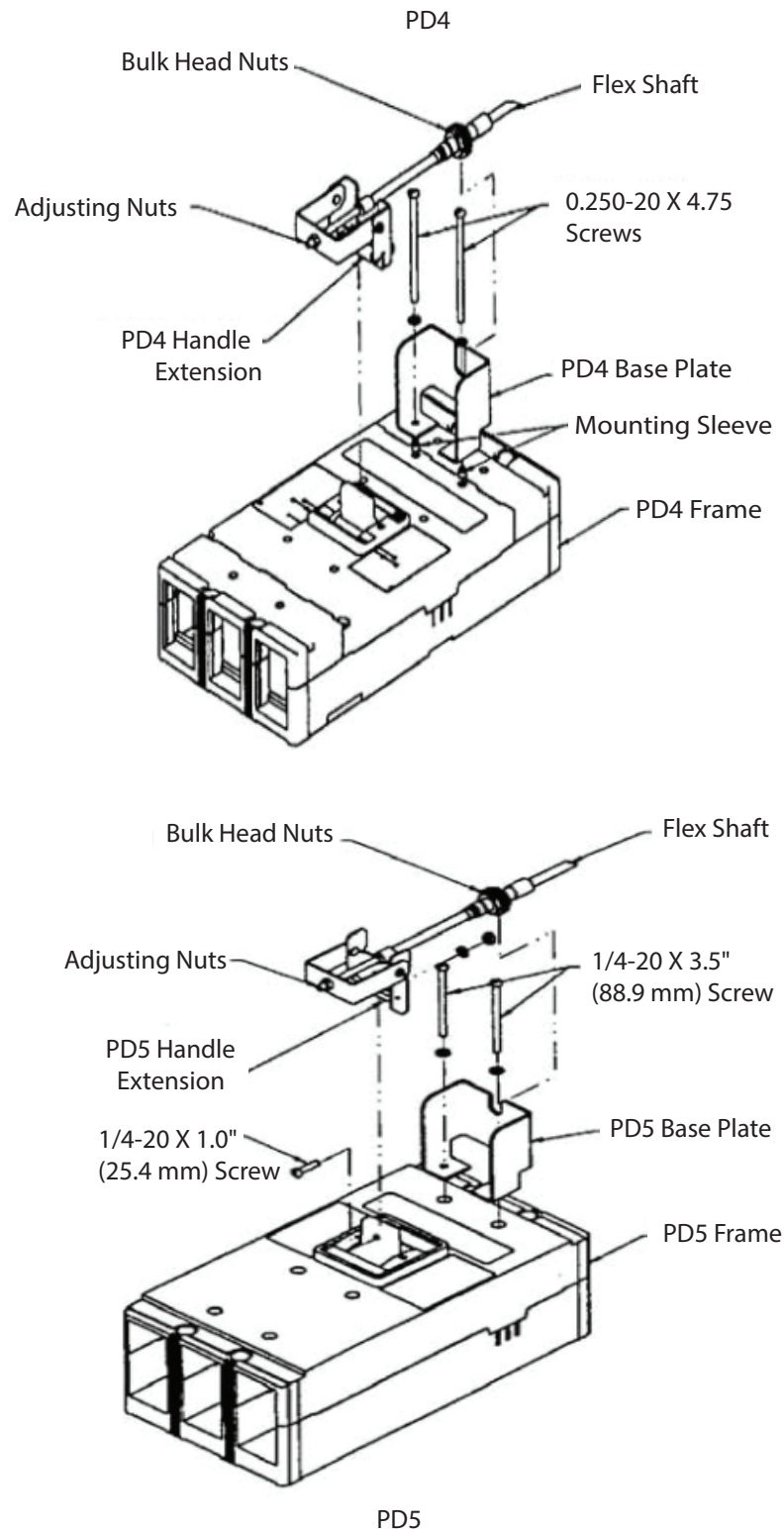
Figure 1-2 PD4, PD5 Mechanism Assembly.
