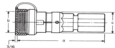
Fig. 8 - NPR Cord Connectors
