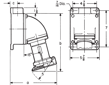
Fig. 3 - 60 and 100 A Receptacle Assemblies
