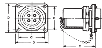
Fig. 6 - NPQ Motor Plugs
