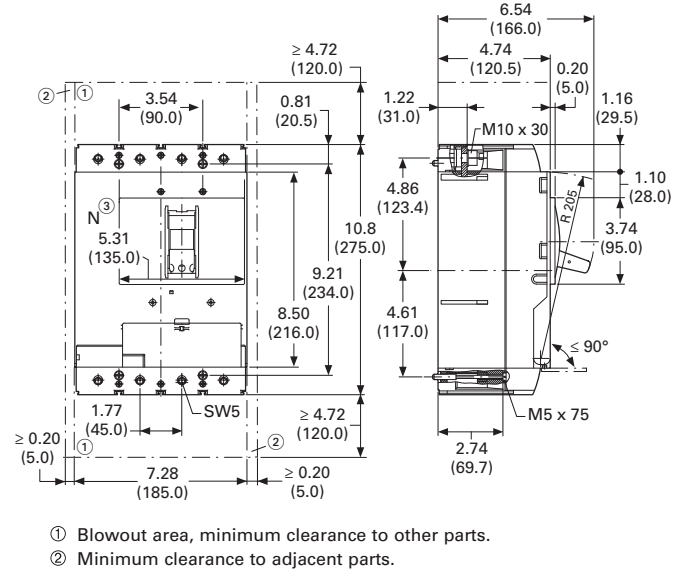
Switch Disconnectors, Four-Pole, N3-4...DC
