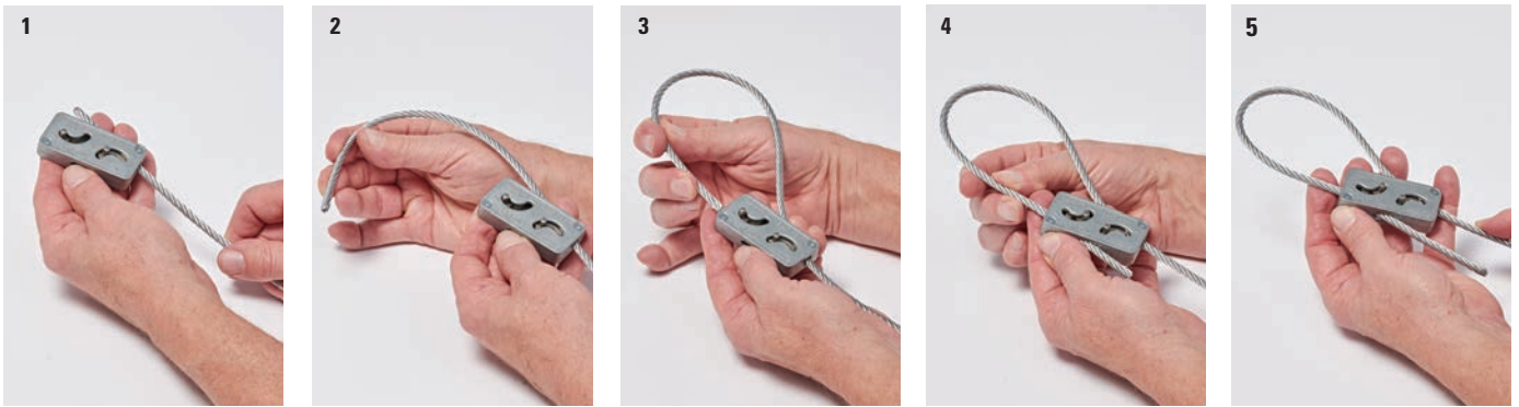
1 Pass the wire rope through the KwikWire Clamp
