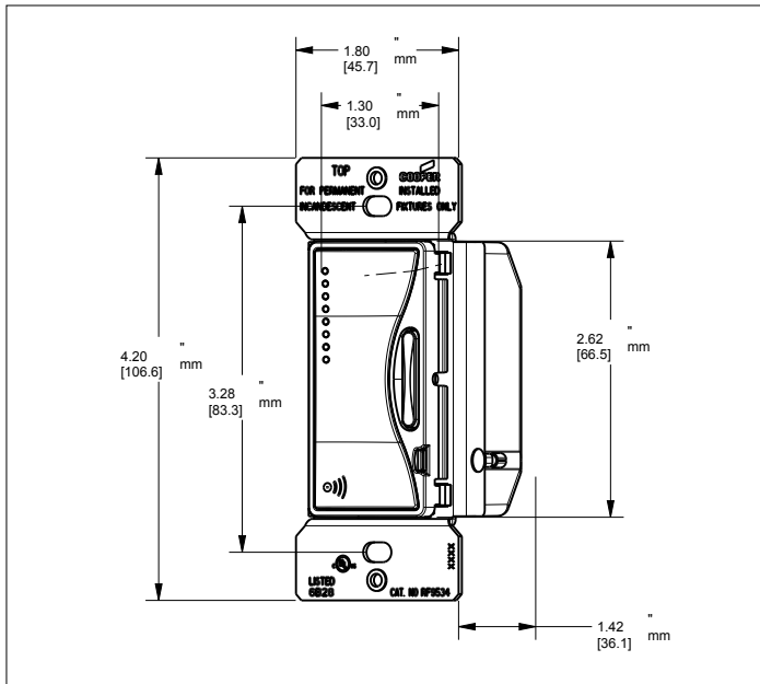
Figure 1. RF9534, RF9536
