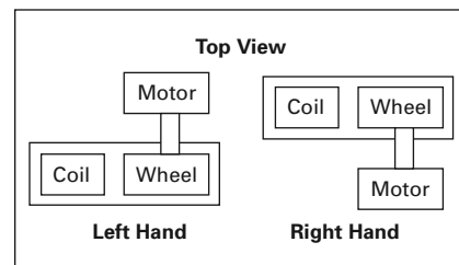
Figure 3. Brake Orientation
