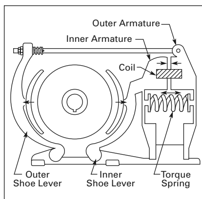
Figure 1. Energized Coil
