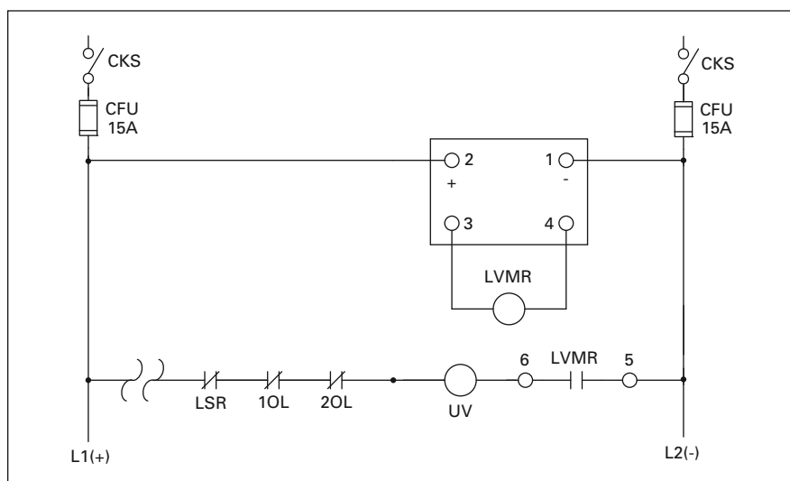
Figure 32. Low Voltage Monitoring Relay Diagram
