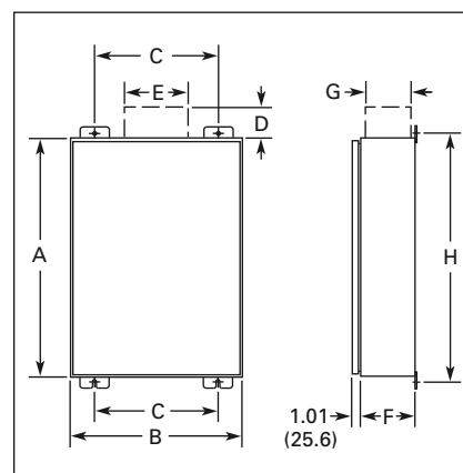
Figure 7. Approximate Dimensions
