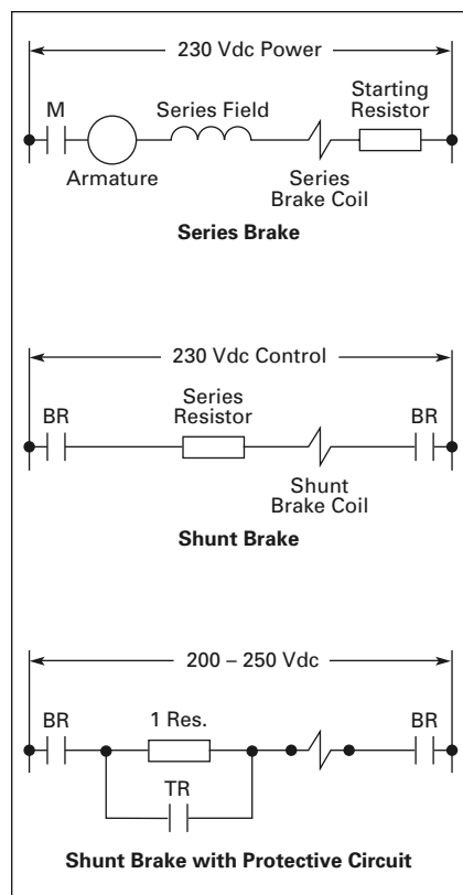
Figure 11. Elementary Diagrams for Standard Brake Circuits
