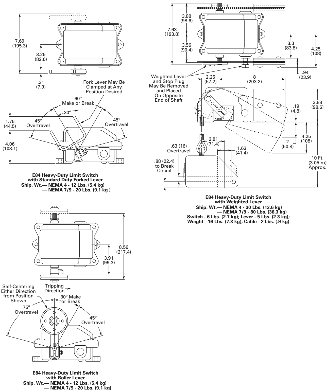
Figure 20. Approximate Dimensions in Inches (mm) and Shipping Weights
