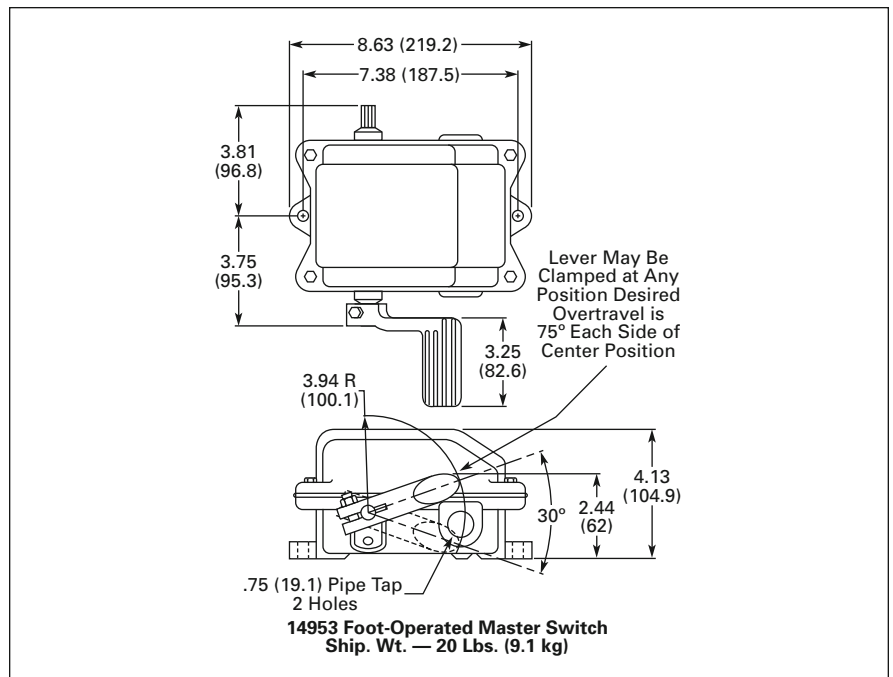
Figure 22. Approximate Dimensions in Inches (mm) and Shipping Weights
