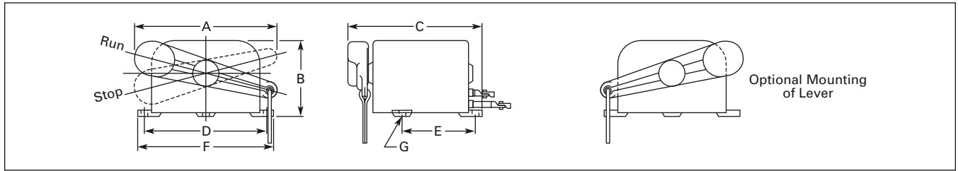
Figure 16. Approximate Dimensions
