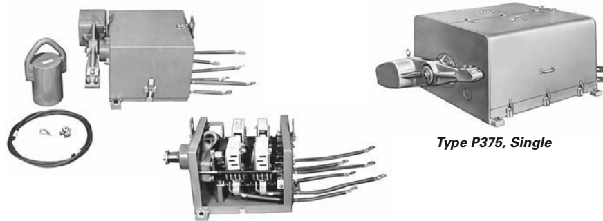
Type P50 Power Limit Switch with Lever, Cable, Fittings and Weight
