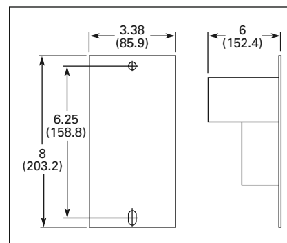
Figure 31. Approximate Dimensions in Inches (mm)
