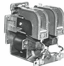
Type KD — NO Pole 2-Pole 50 A
