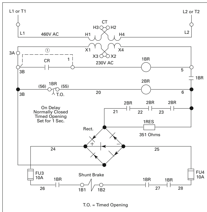
Figure 6. Elementary Diagram
