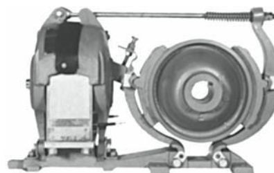
GH505 Magnetic Shoe Brake
