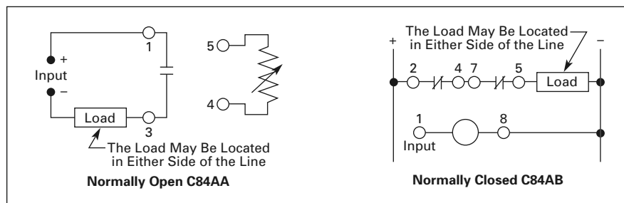
Figure 30. Wiring Diagrams
