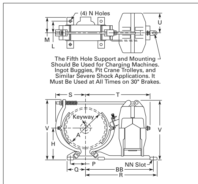
Figure 8. Brake Dimensions
