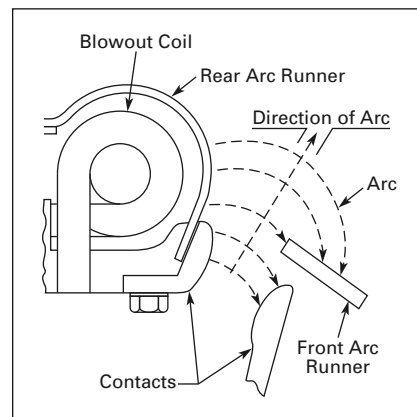
Figure 26. Blowout Coil Effect on Arc
