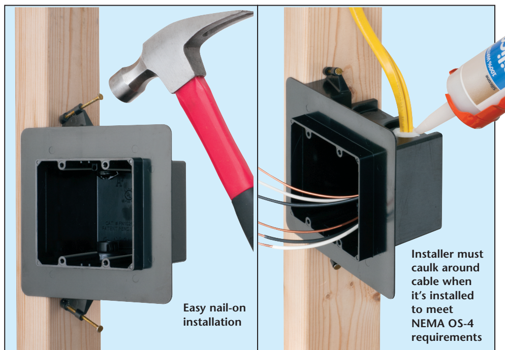
Captive nails
