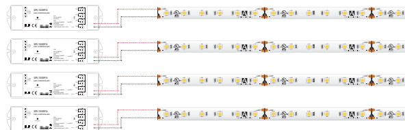
Trulux RF Receivers (Receiver required per zone)
