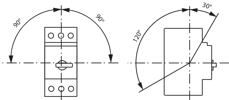
Mounting position
