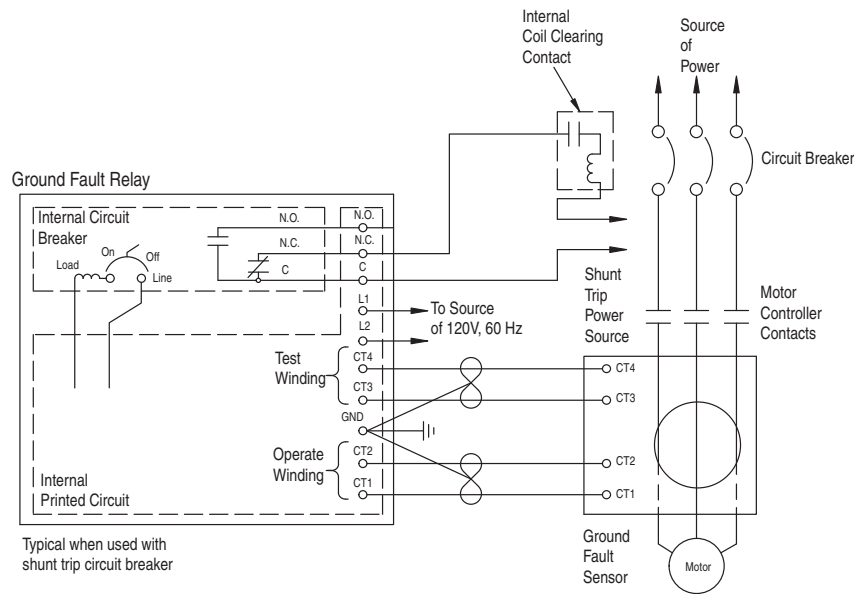
Figure 2 - Class II with High Current Inhibit Circuit (1)
