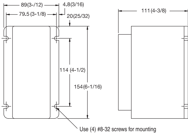
Figure 4 - Arcing Ground Fault Sensors
