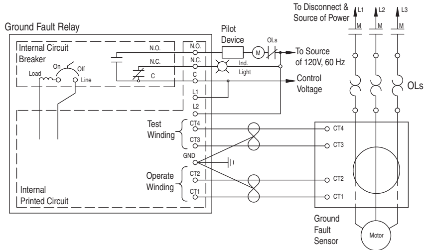
Figure 2 - Class II with High Current Inhibit Circuit (1)
