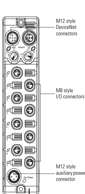
Plastic housing
