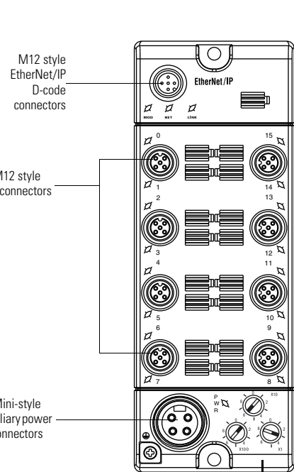
Metal housing
