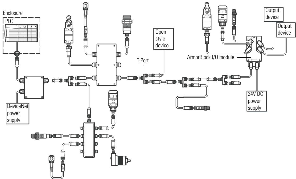
DeviceNet Thin Round Trunk Configuration Example
