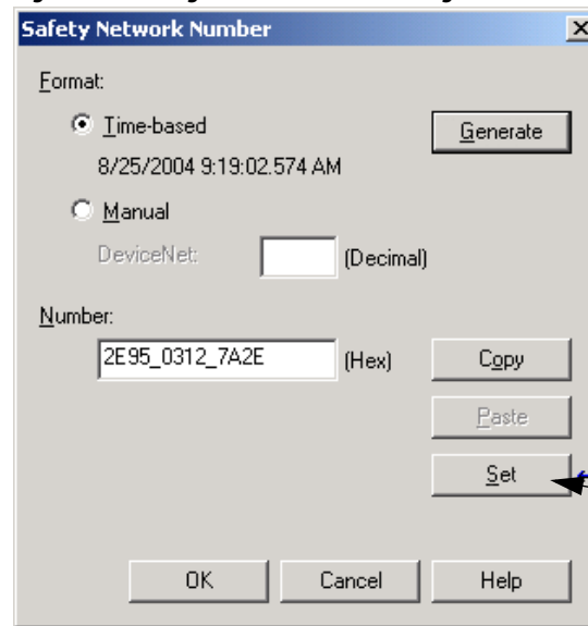
Figure 46 - Setting the SNN with a GuardLogix Controller
