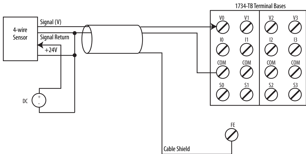
Figure 42 - 4-wire Voltage or Tachometer Sensor (SIL 2) with External Power Supply
