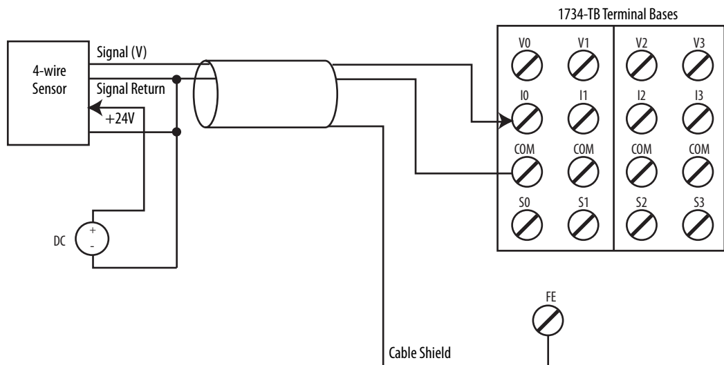
Figure 43 - 4-wire Current Sensor (SIL 2) with External Power Supply
