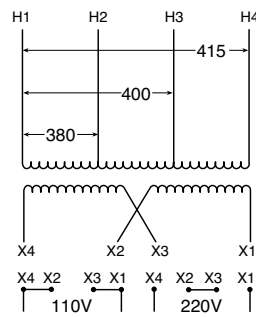
WIRING FOR AE 12
