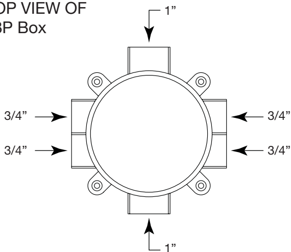
FIGURE 2 Conduit Sizes
