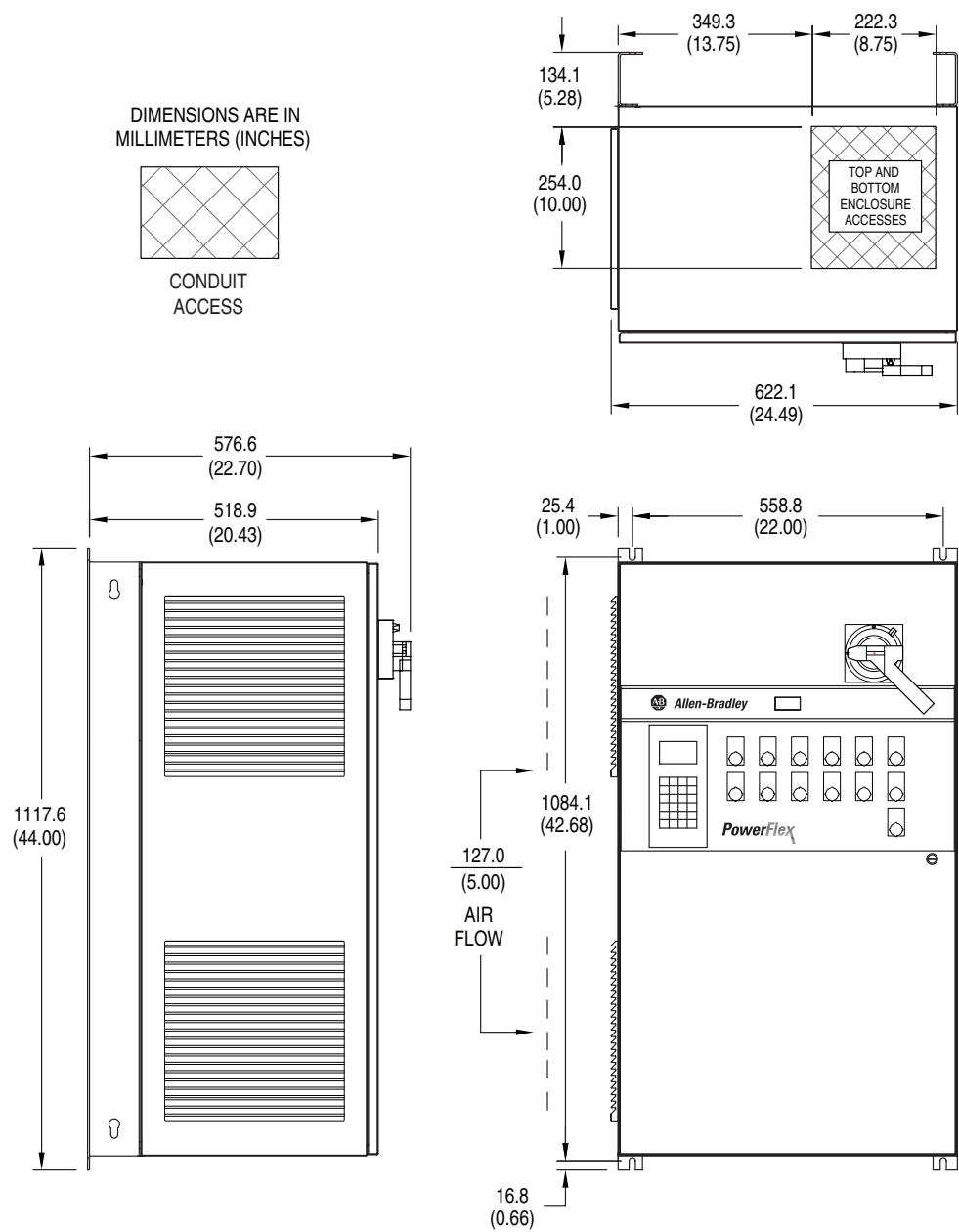
Figure 6. PowerFlex 700 6 Pulse, Frame 2, NEMA/UL Type 12
