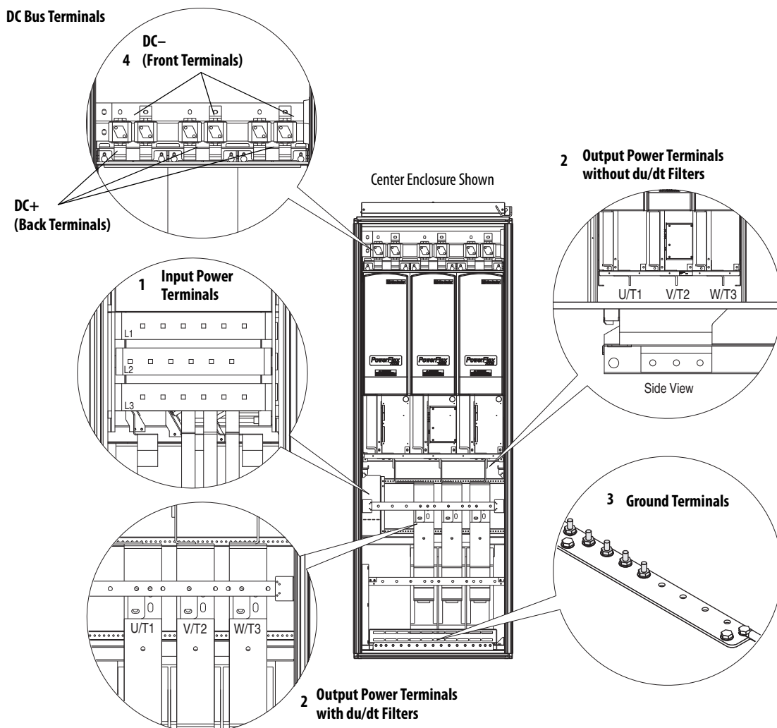
Figure 64 - 1500A Drive Power Terminal Locations
