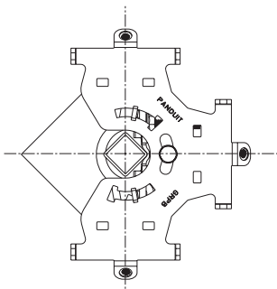
\frac{7}{8} " (22.2mm) Square Pedestal (mounted at 45°)
