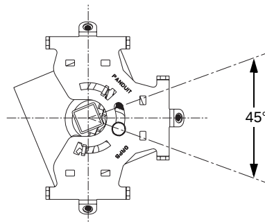
\frac{7}{8} " (22.2mm) Square Pedestal (mounted off center)
