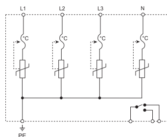
TNS Configuration
