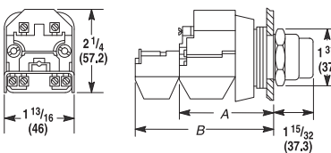
Transformer Type (Push-to-test Pilot Light and Illuminated Push Button)
