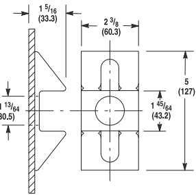
Ramp Guard for Push-pull Illuminated or Non-illuminated Operators
