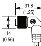
Figure F Right Angle Female
