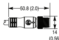
Figure G Straight Male
