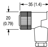
Figure G Micro Right Angle Female
