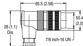
Figure D Micro Style Male
