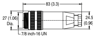
Figure A Mini Style Female
