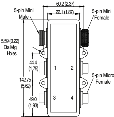
4-port micro thru-trunk DevicePort
