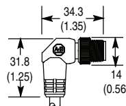
Figure H Right Angle Male
