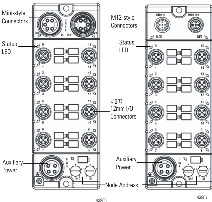
1732D-IB16M12MINI shown
