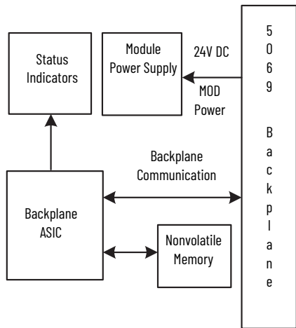
5069-ARM Functional Block Diagram
