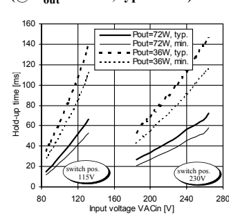
Hold-up time with ACin (@ V_{out} = 24.5\text{V} , typ. + min.)
