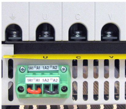
Drive with no fan
