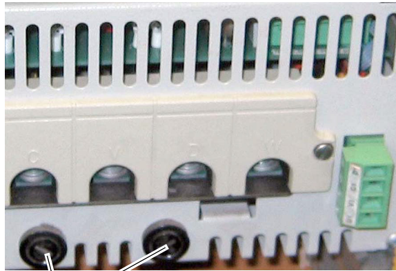
Bottom View of Drive without Fan
