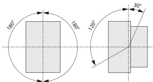
Figure 74 - 100-E116K..., 100-E146K... Contactors
