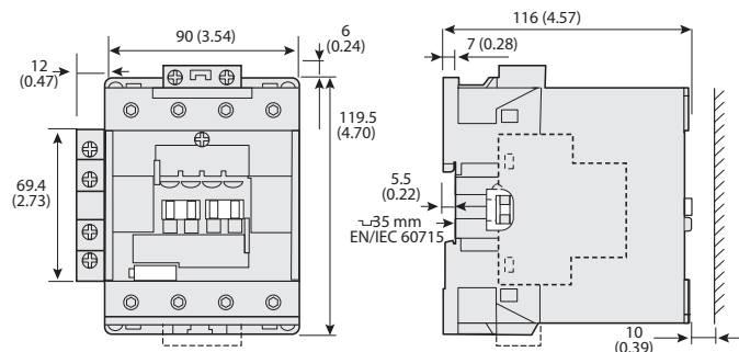
Figure 71 - 100-E80 4-Pole Contactors with Side-mounted Auxiliary Contact
