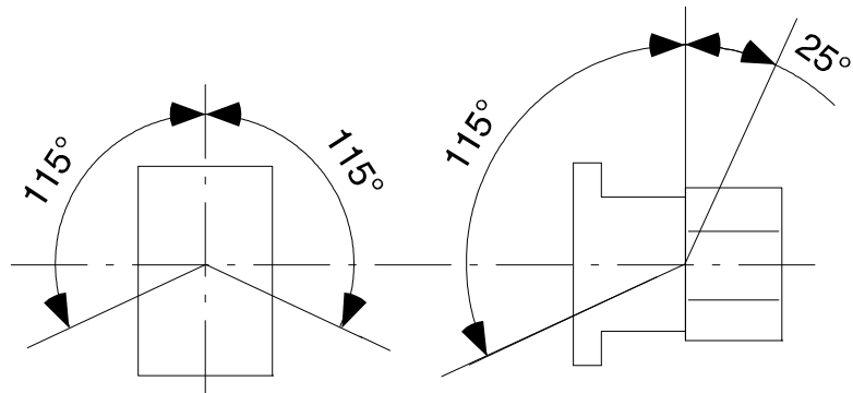
Figure 25 - Mounting Position – 100S-C DC Contactors with Conventional Coils
