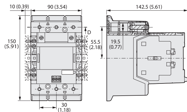
Figure 75 - 100-E116E..., 100-E146E... Contactors with PLC Input
