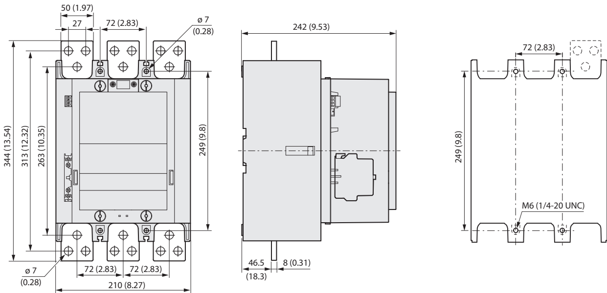
Figure 89 - 100-E860, 100-E1060, 100-E2050, 100-E2650 Contactors with PLC Input
