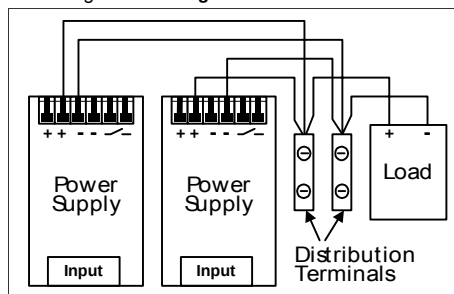
Fig. 27-9 Using distribution terminals
