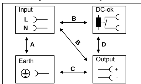
Fig. 20-1 Dielectric strength
