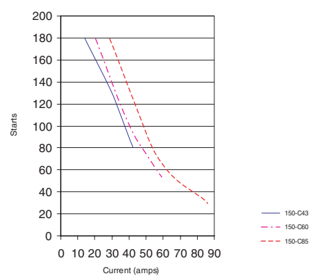
SMC-3 Starts per hour (14-85A) 40C, 100% Duty Cycle, 20sec, 350% (with standard fan)
