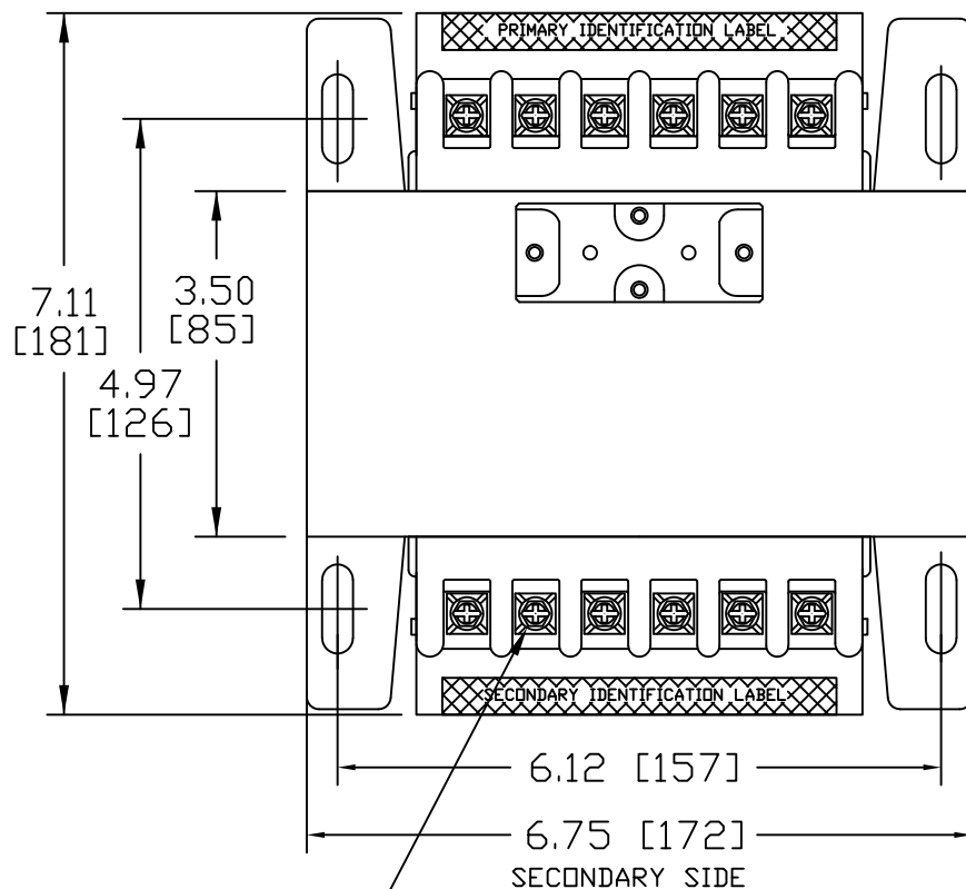
PRIMARY SIDE
