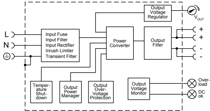
Fig. 11-1 Functional diagram
