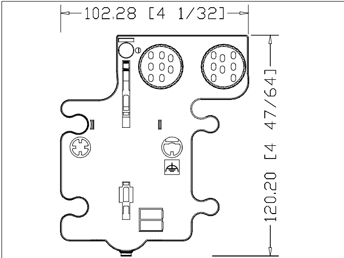
1738-Mounting Base I/□
