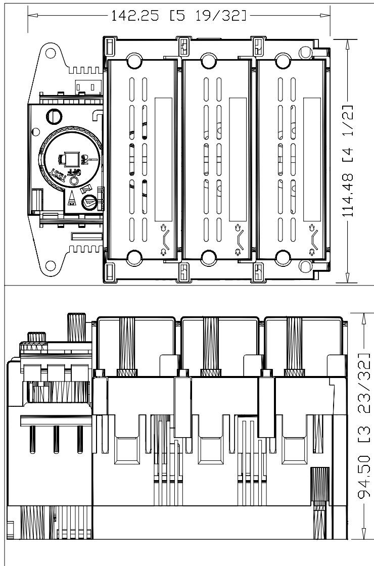
194R-N60-1753* 194R 60 Amp Non-fused Disconnect, 3-Poles
