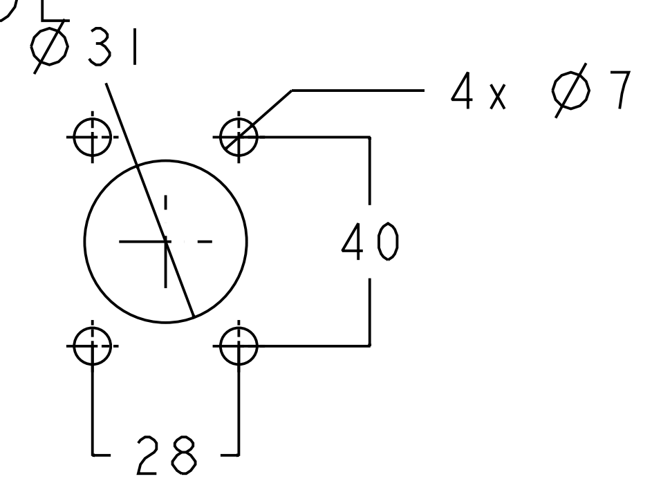
BOX DRILLING SIDE
