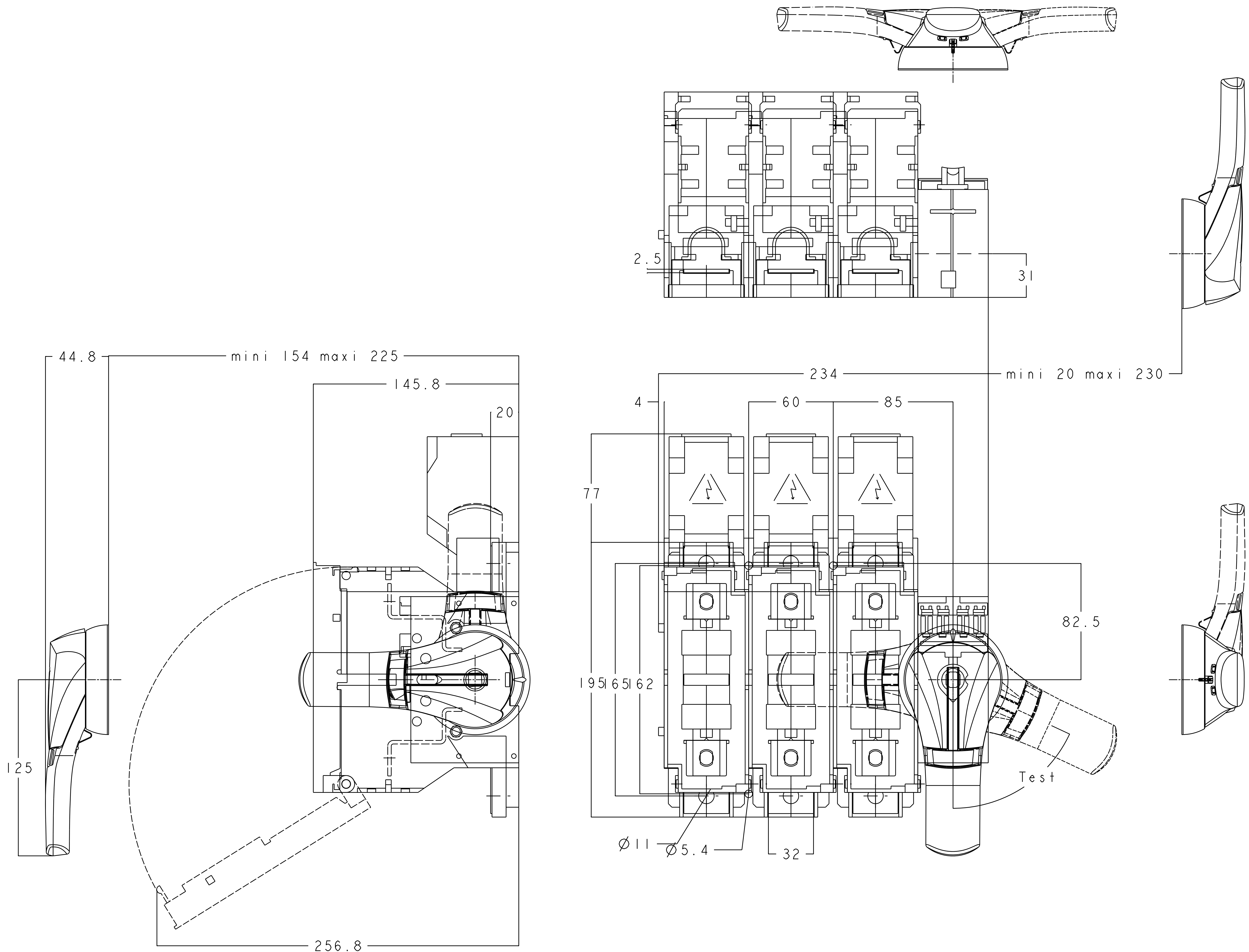
BOX DRILLING SIDE
