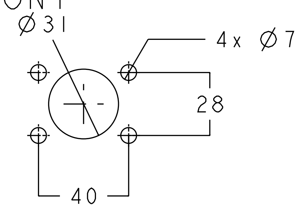
DOOR DRILLING FRONT
