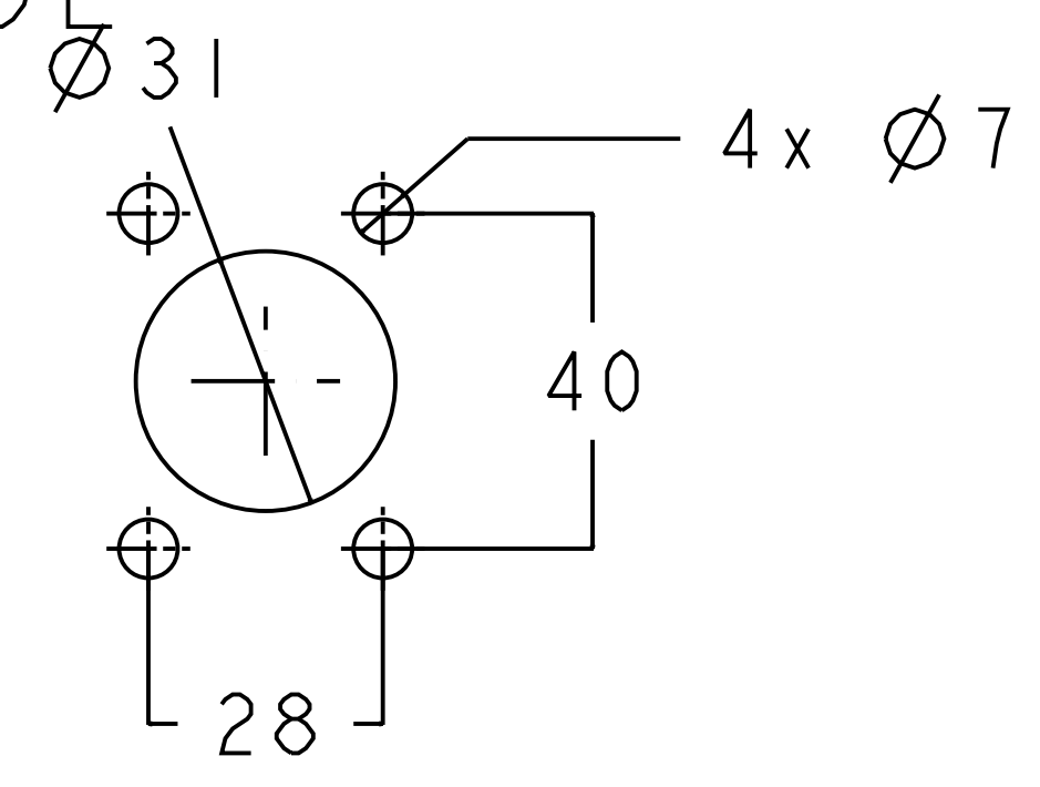
BOX DRILLING SIDE
