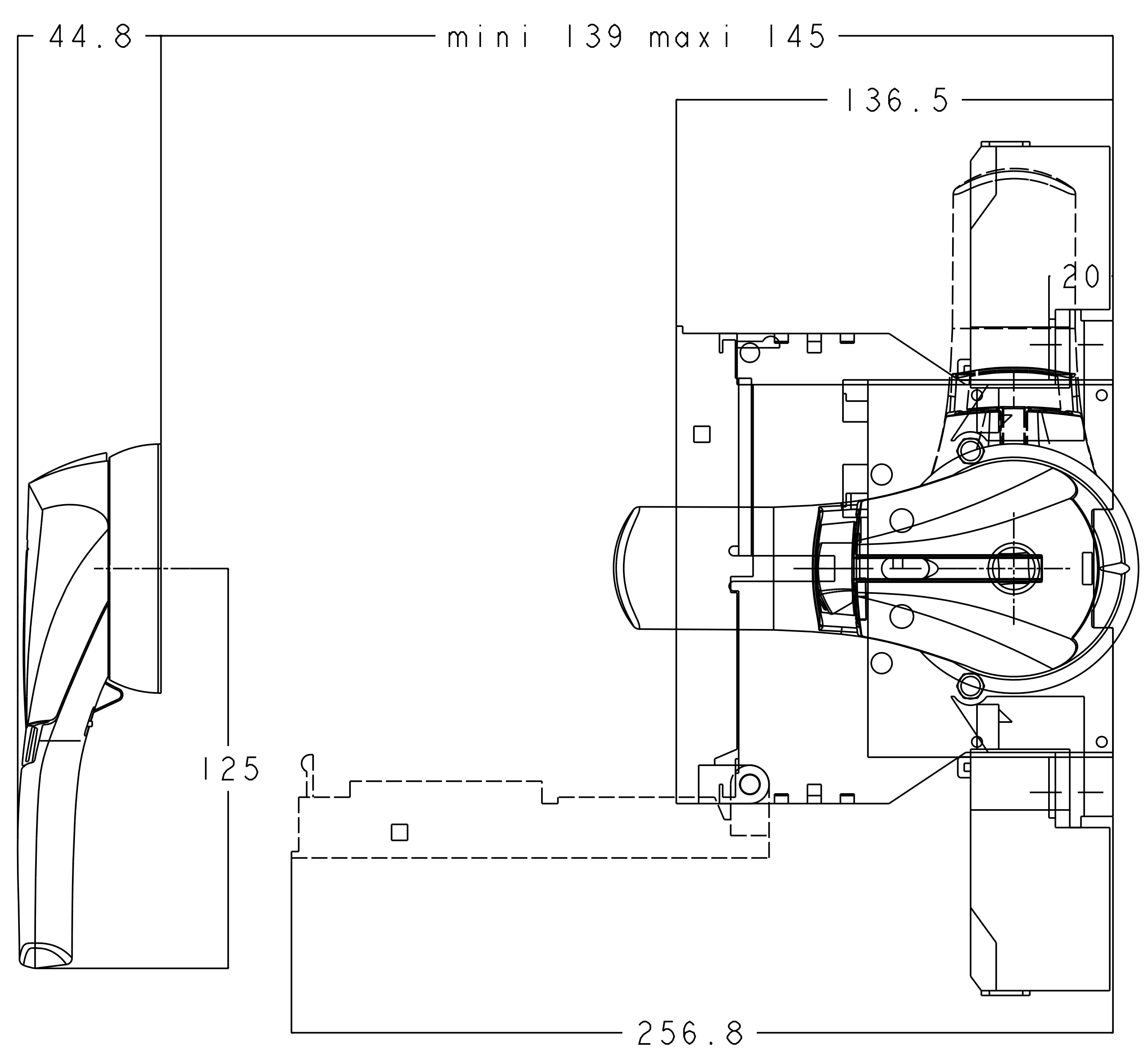
BOX DRILLING SIDE
