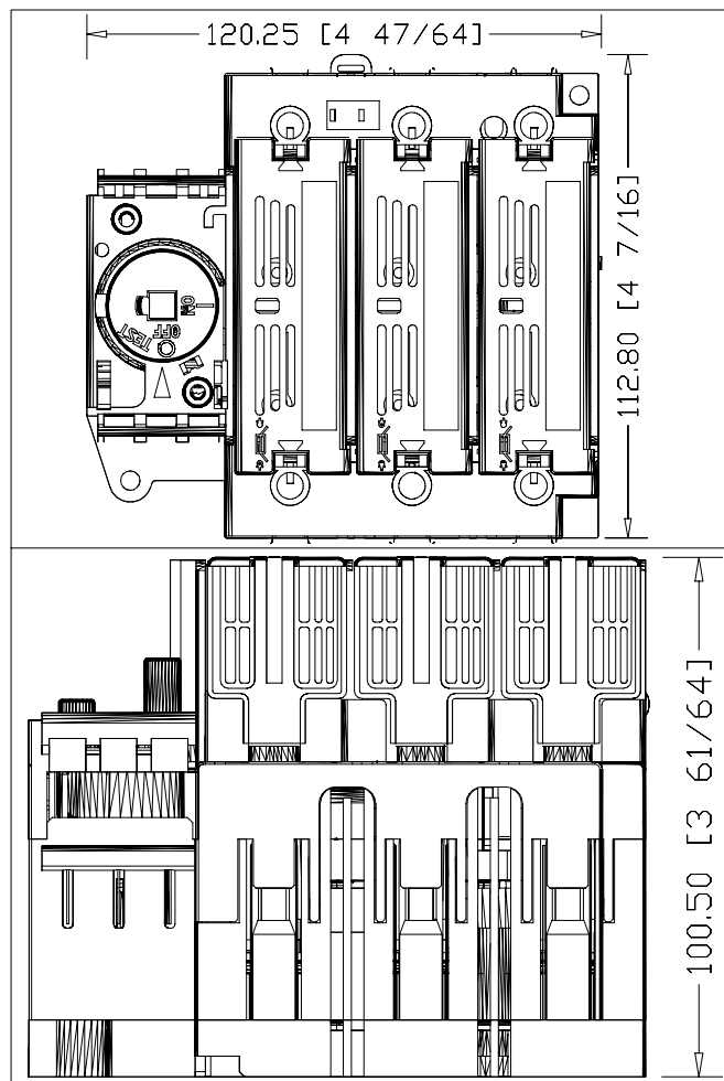
194R-F25/F32-1753* 194R 25/32 Amp Fused Disconnect (NFC), 3-Poles
