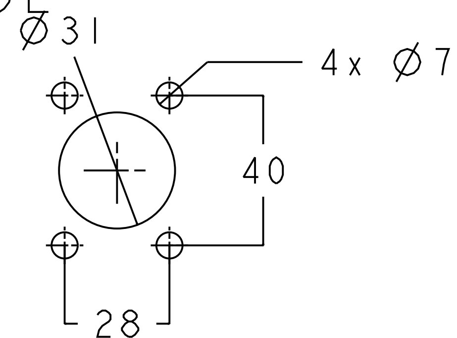
BOX DRILLING SIDE
