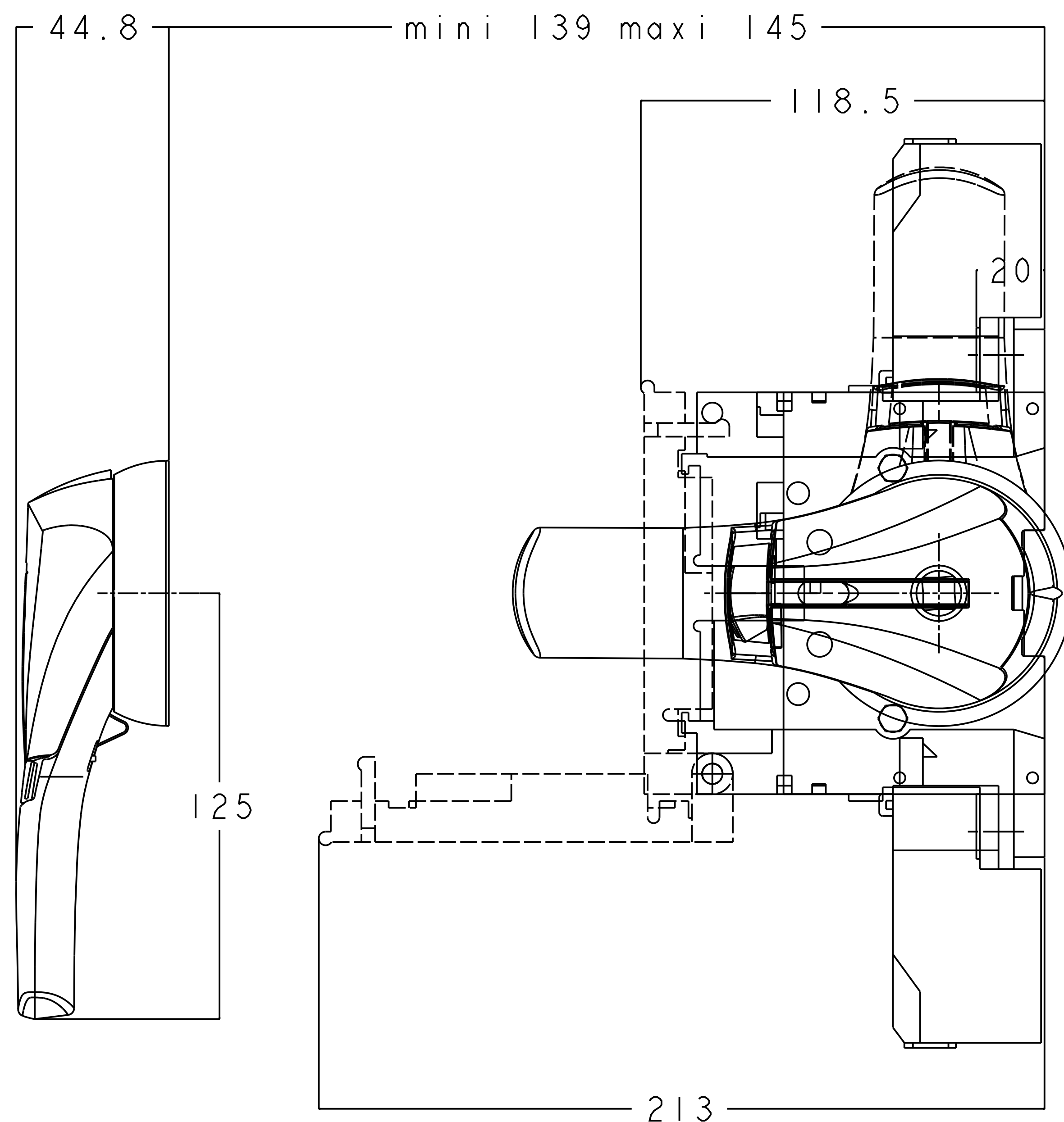
BOX DRILLING SIDE
