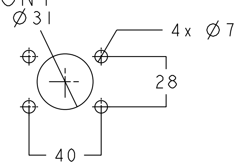
DOOR DRILLING FRONT
