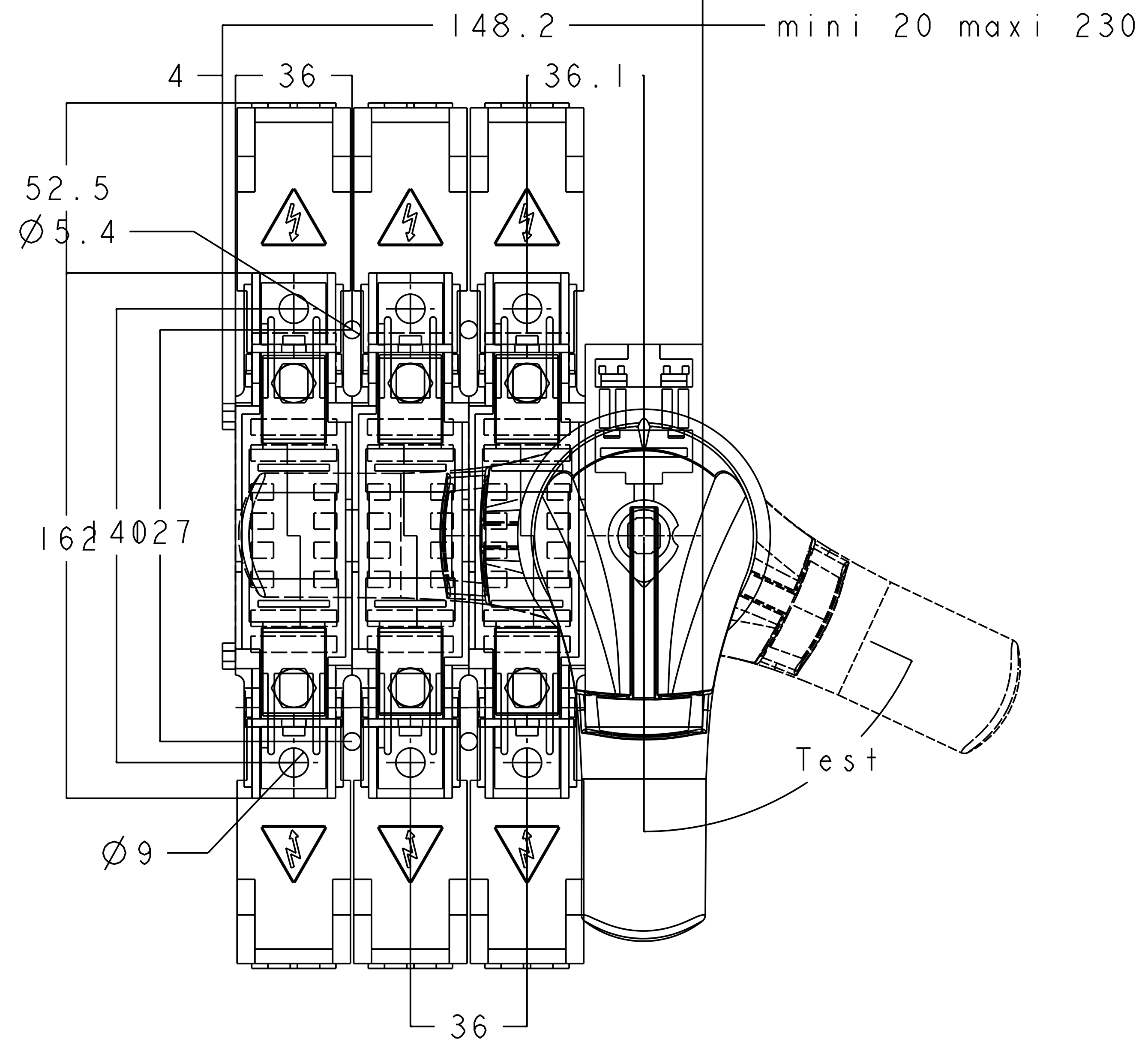
DOOR DRILLING FRONT
