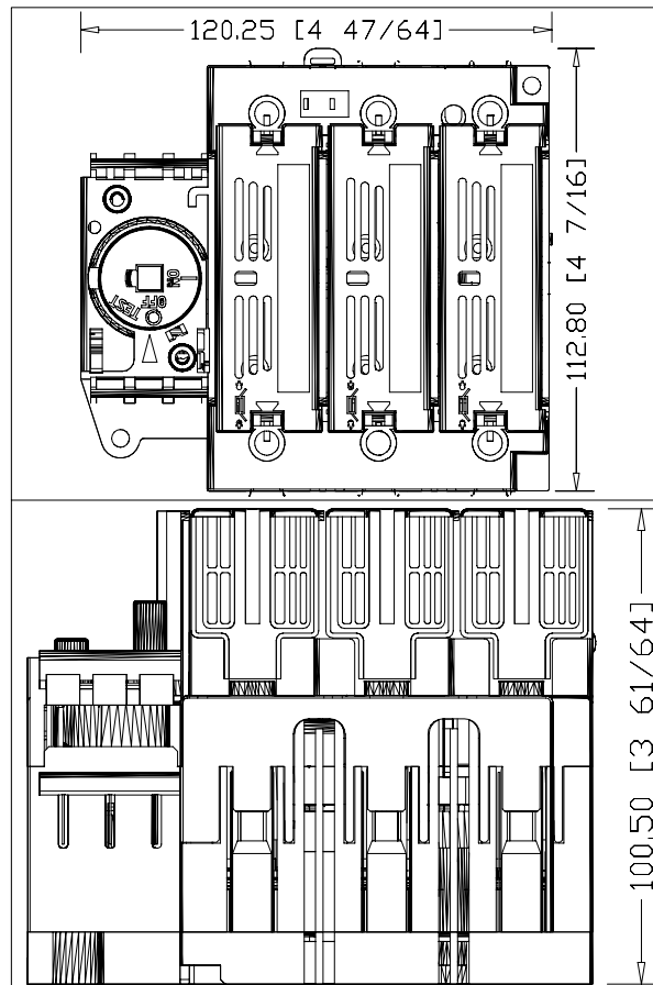
194R-J30-1753* 194R 30 Amp Fused Disconnect (J), 3-Poles
