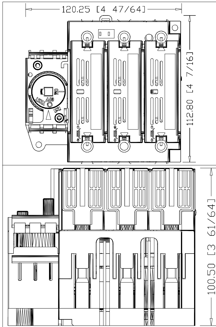
194R-H30-1753* 194R 30 Amp Fused Disconnect (HRCII-C), 3-Poles
