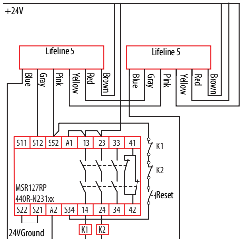
MSR127RP with 1 Sensor, Monitored Manual Reset, Driving 100S or 700S Safety Relays.
