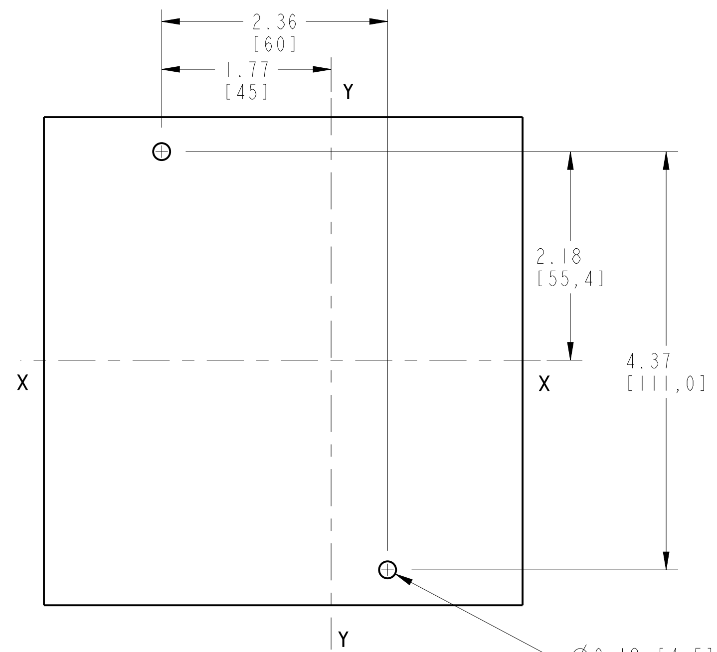
DRILLING FOR FIXING CIRCUIT BREAKER SCALE 1:1
