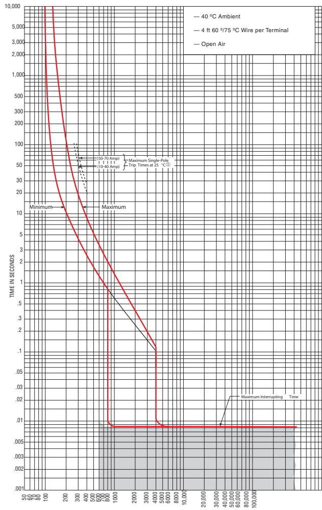
Time Current Curve — 1-Pole Circuit Breaker
