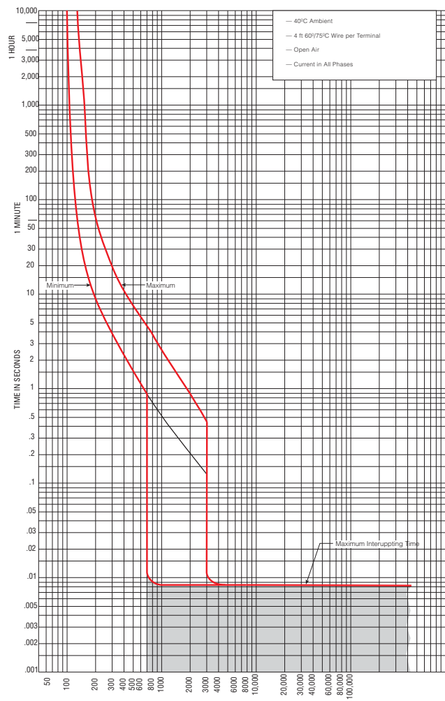
Time Current Curve — 3-Pole Circuit Breaker
