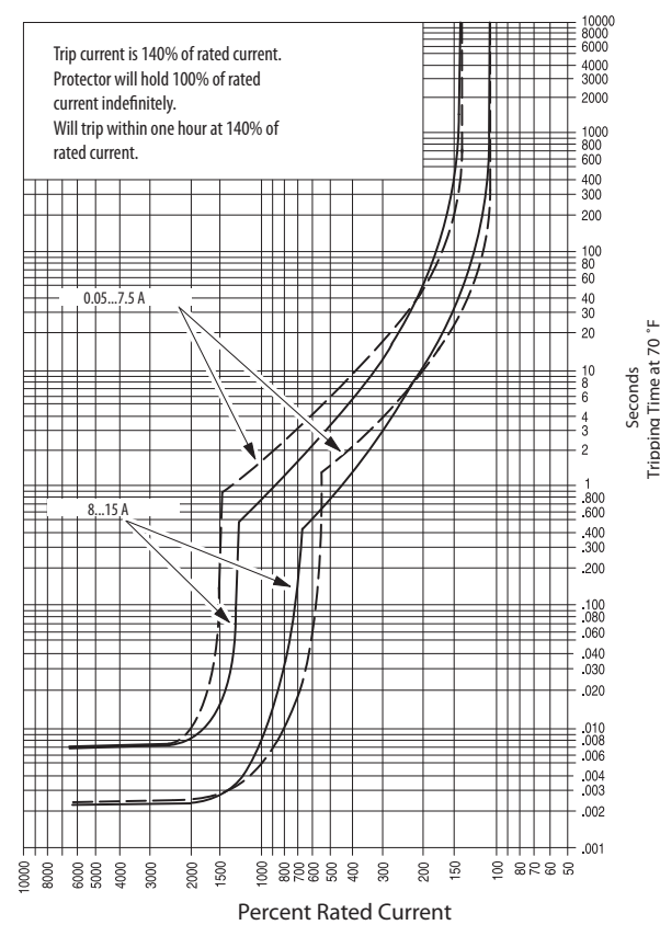
Time Current Curve -1492-GH
