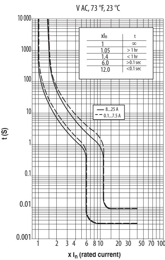
Time Current Curve -1492-GS
