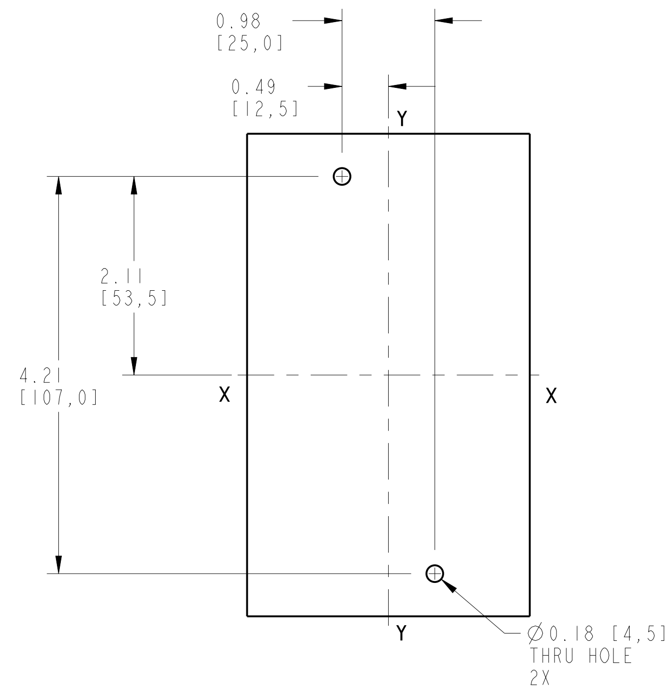
DRILLING FOR FIXING CIRCUIT BREAKER SCALE 1:1
