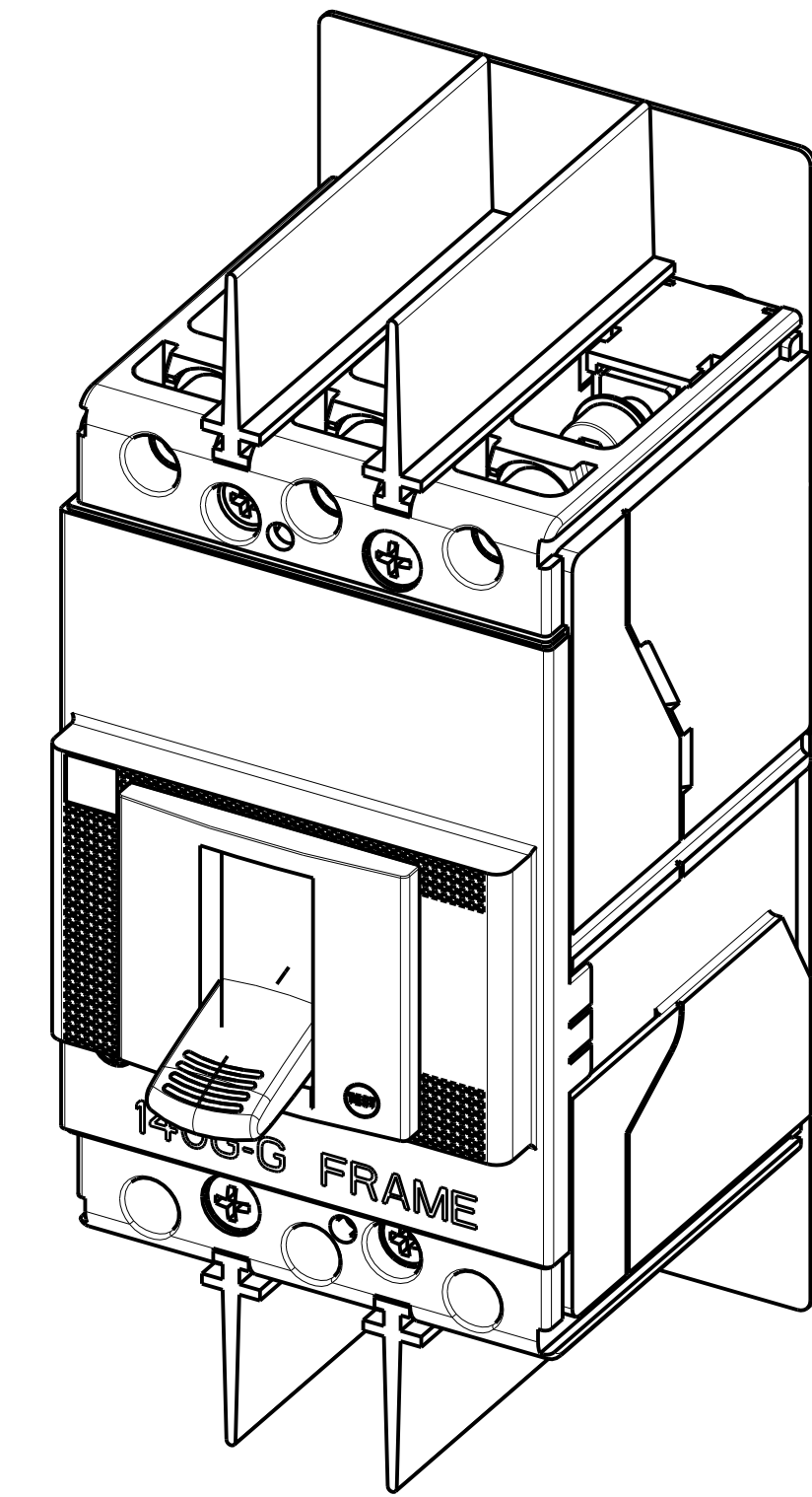
ISOMETRIC VIEW
