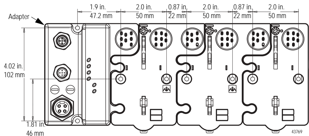
Drilling dimensions
