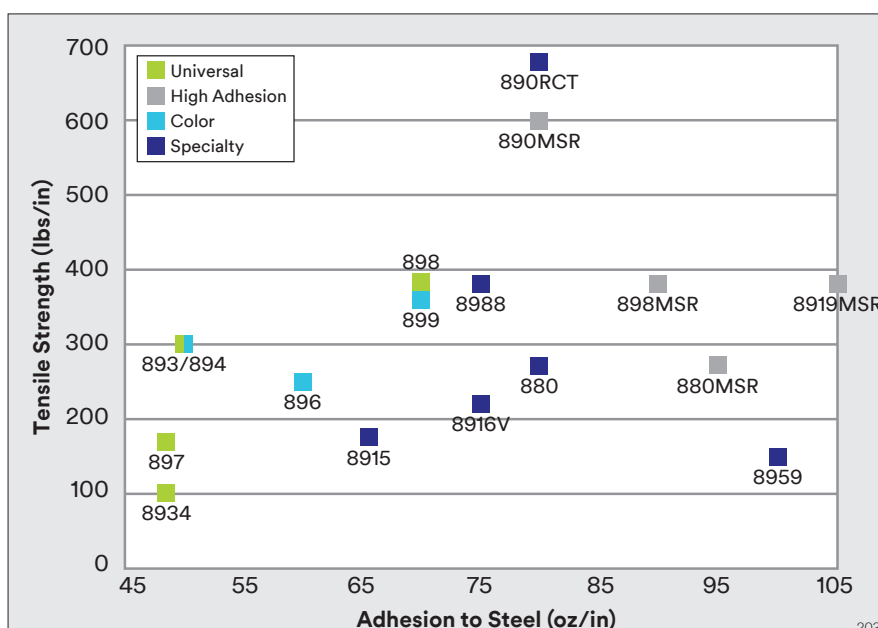
Performance Map — Filament Reinforced Tapes
