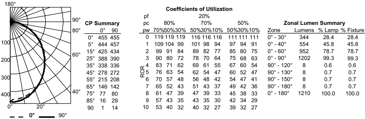
FMLWL 24 840, 1,200 delivered lumens
