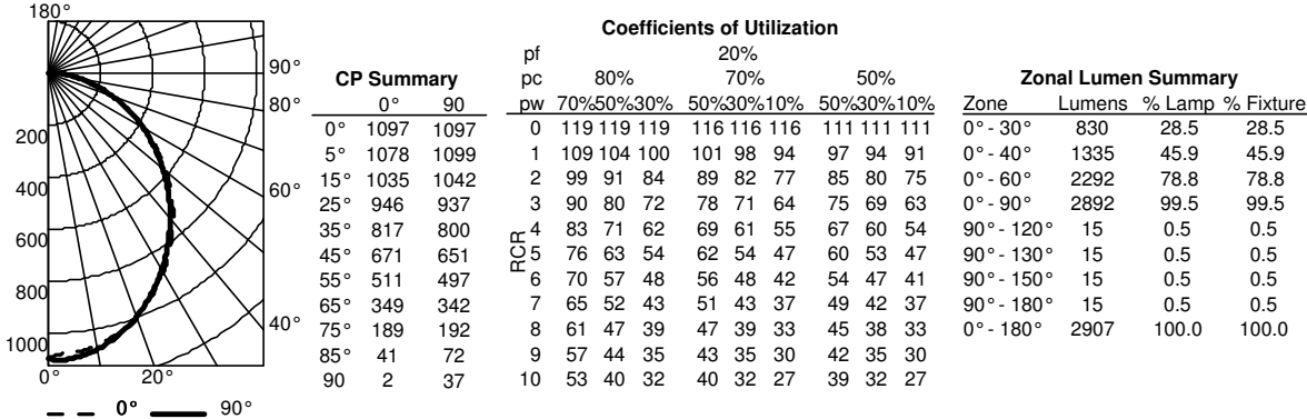
FMLWL 48 840, 2,900 delivered lumens
