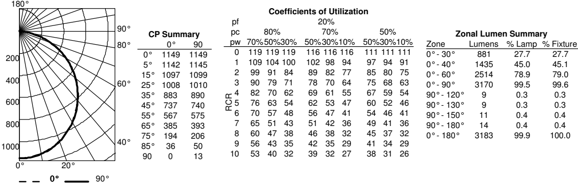
FMLWL 24 840 ZT MVOLT, 3,186 delivered lumens
