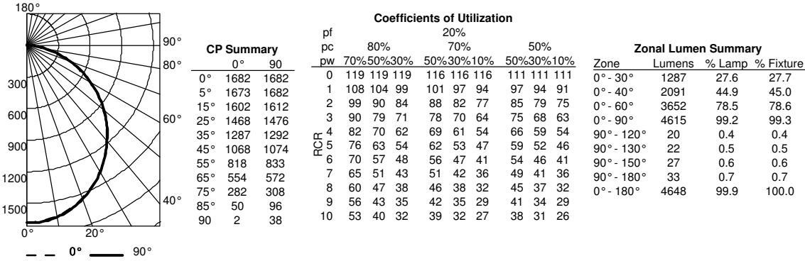
FMLWL 48 840 ZT MVOLT, 4,654 delivered lumens
