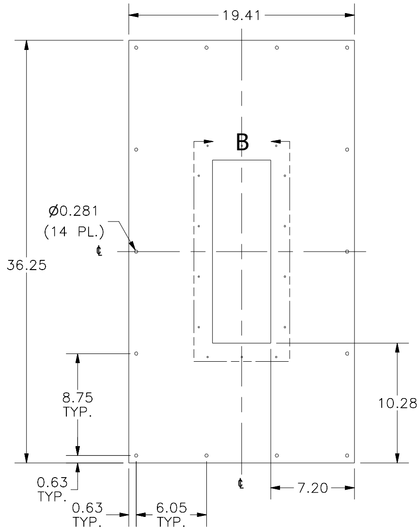
FRONT VIEW (PLATE ONLY)
